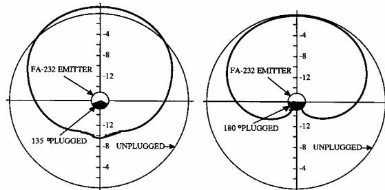
Directivity Patterns for Plugged FA-232/FA-390 Fog Horns
